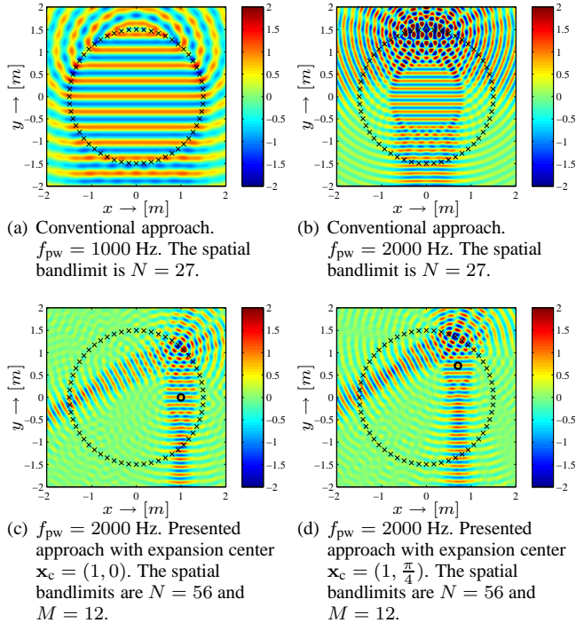
Fig. 3. Wave fields reproduced by a circular distribution of L = 56 discrete loudspeakers and with radius r_0 = 1.5 m reproducing a plane wave with propagation direction \theta_{pw} = \frac{3\pi}{2} . The marks indicate the positions of the secondary sources.
