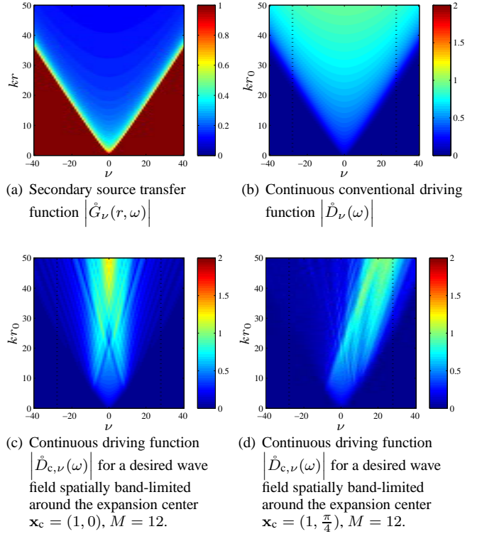
Fig. 2. Absolute values of the Fourier coefficients with respect to the expansion around the origin of the global coordinate system. The black dotted lines indicate the interval of one spectral repetition due to spatial sampling. kr_0 = 50 corresponds to f \approx 2700 Hz.
