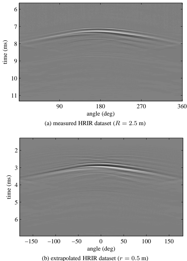
Fig. 3: Measured and range extrapolated HRIR dataset for the left ear ( \alpha = 180^\circ ).
