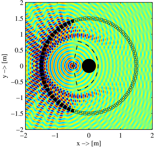
Fig. 2: Synthesis of a focused source with WFS using a circular loudspeaker array ( N = 72 , R = 1.5 m, f_{fs} = 3 kHz, \mathbf{x}_{fs} = [-0.5 \ 0]^T m, \mathbf{n}_{fs} = [1 \ 0]^T ). The active loudspeakers are filled.
