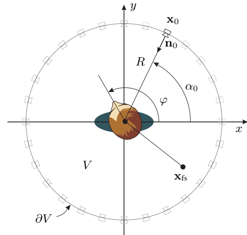
Fig. 1: Geometry used for measurement and range extrapolation of HRIR datasets.
